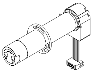
Configuration with fittings 1/4"–28 UNF
